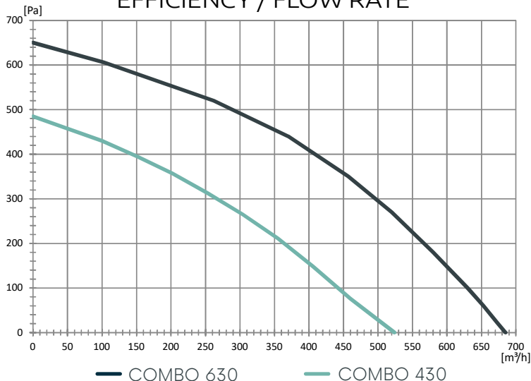
EFFICIENCY / FLOW RATE
