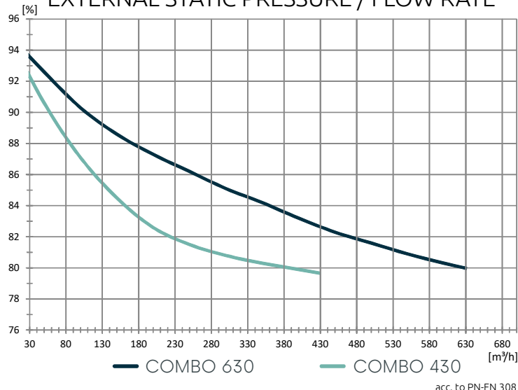
EXTERNAL STATIC PRESSURE / FLOW RATE
